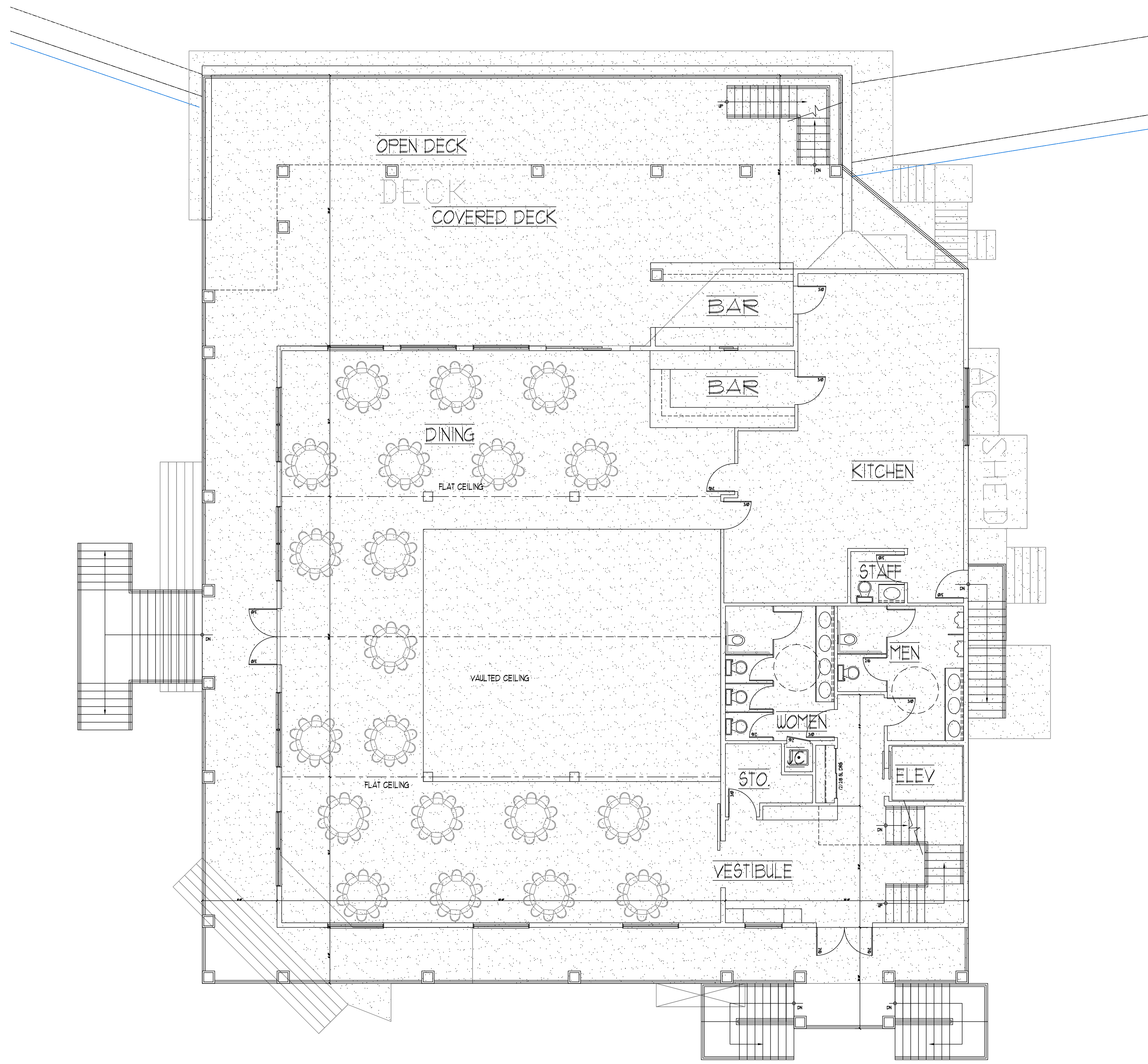
1 MAIN LEVEL OVERLAY SCALE: 3/16" = 1'-0"
